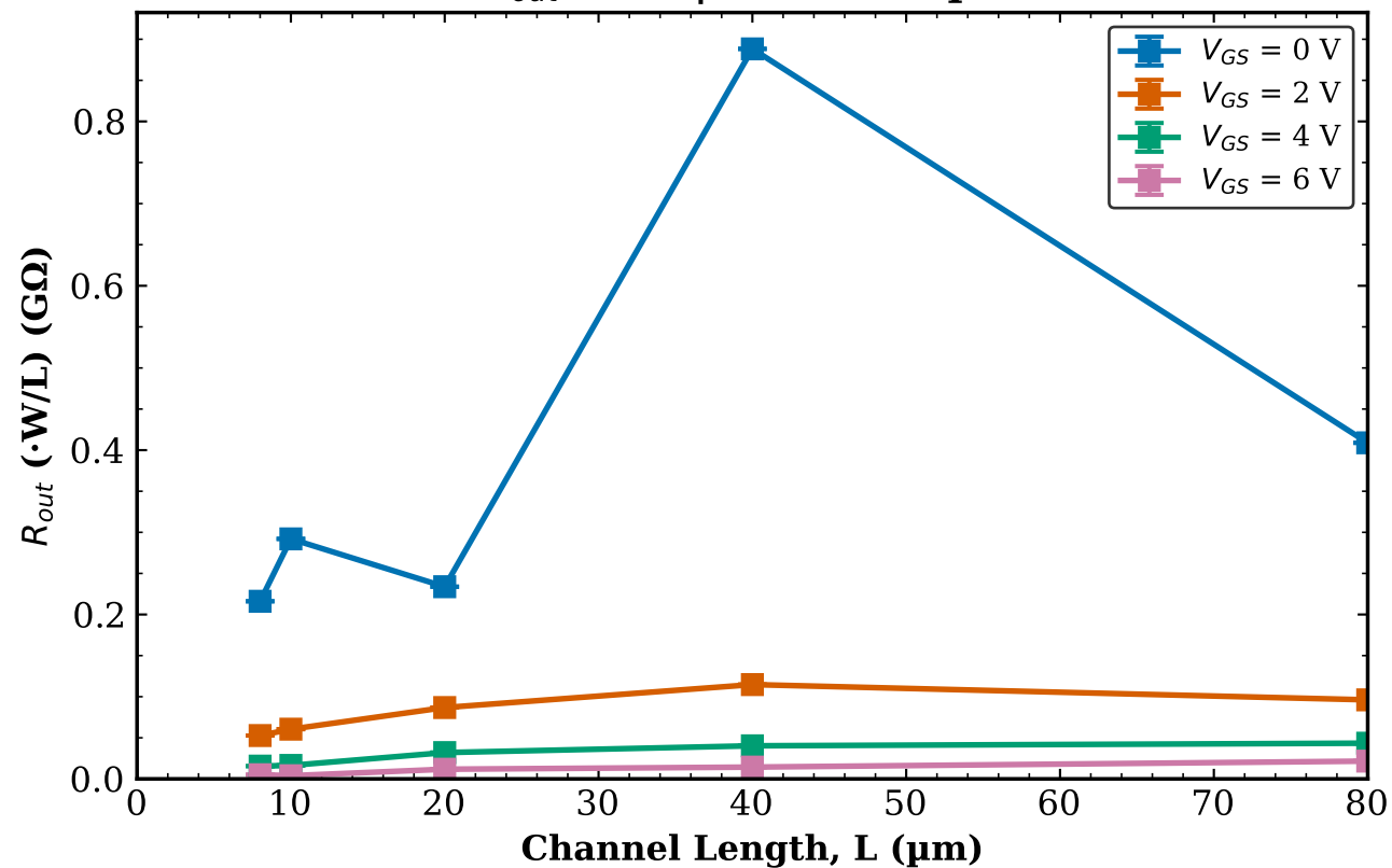
TFT1 Transistor 1 R_{out} vs L | W = 500\text{ }\mu\text{m}
